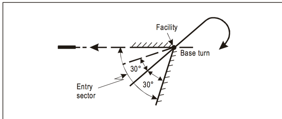
Figure I-4-3-3. Direct entry to base turn
