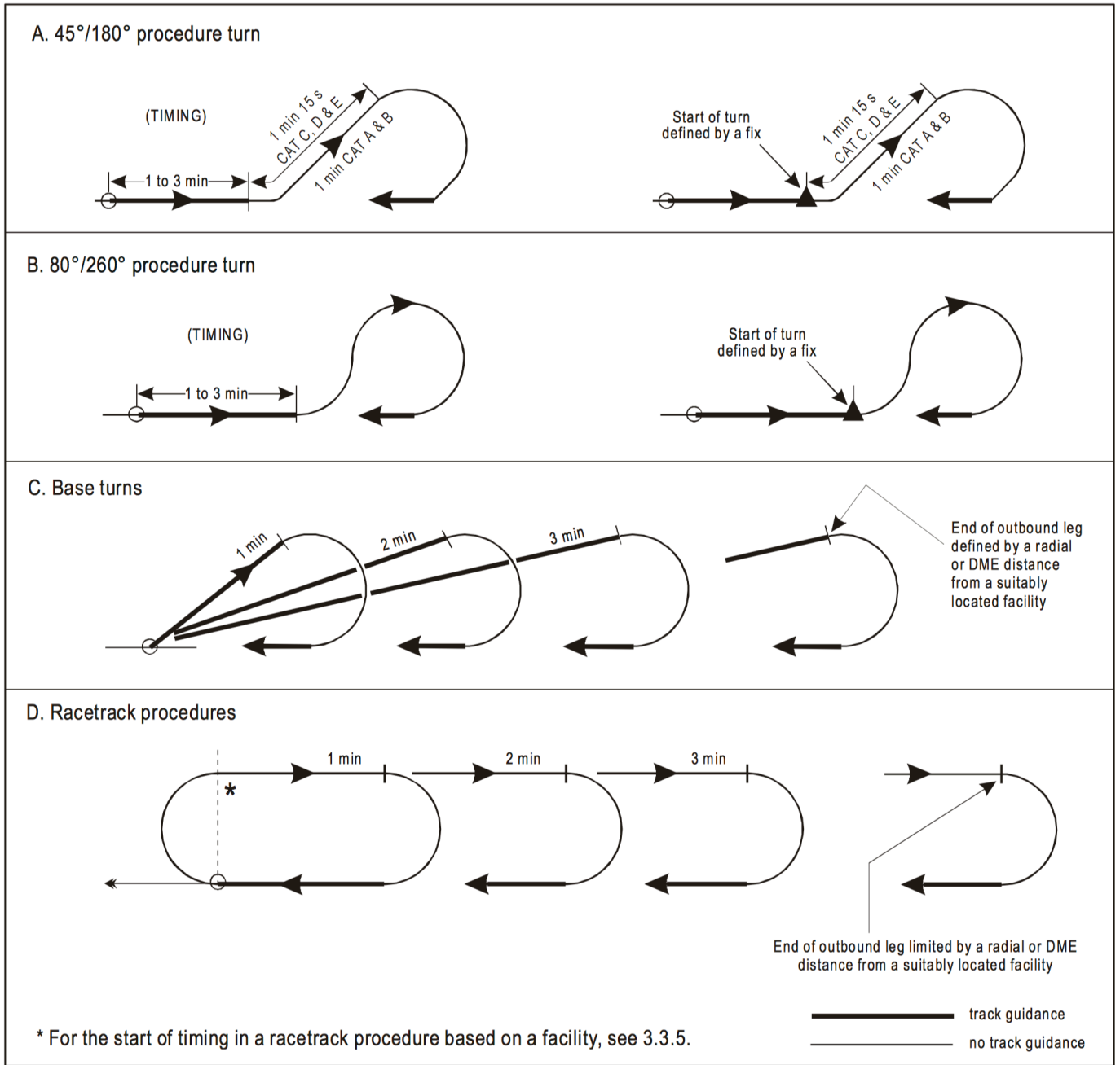
Figure I-4-3-1. Types of reversal and racetrack procedures
