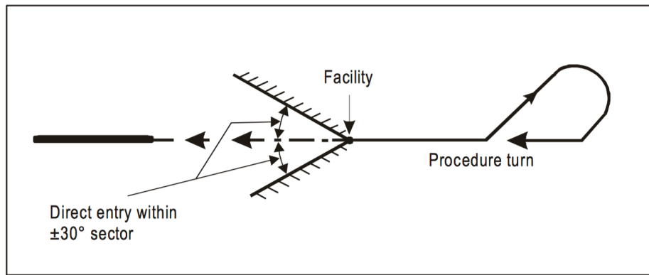
Figure I-4-3-2. Direct entry to procedure turn
